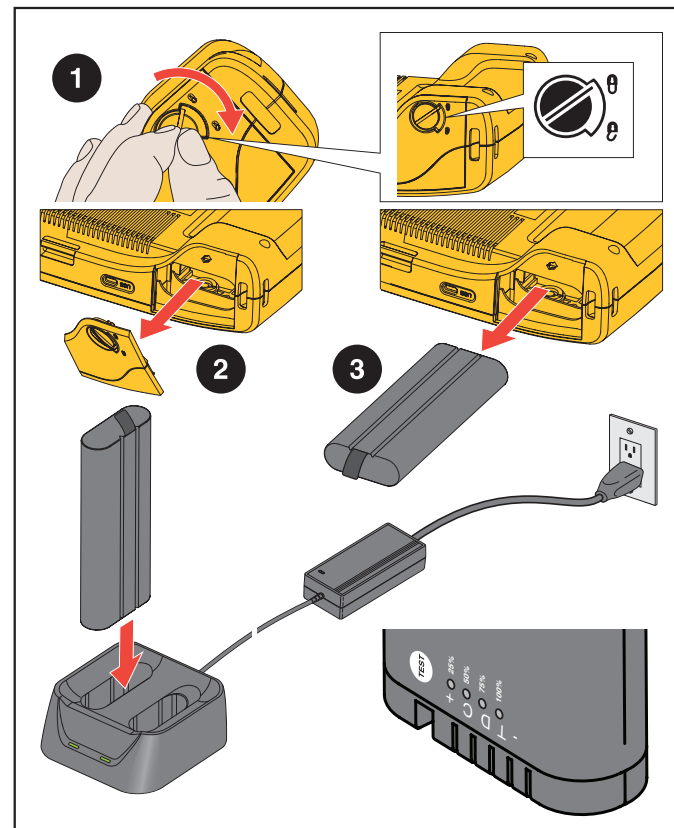
Figure 1. Battery
