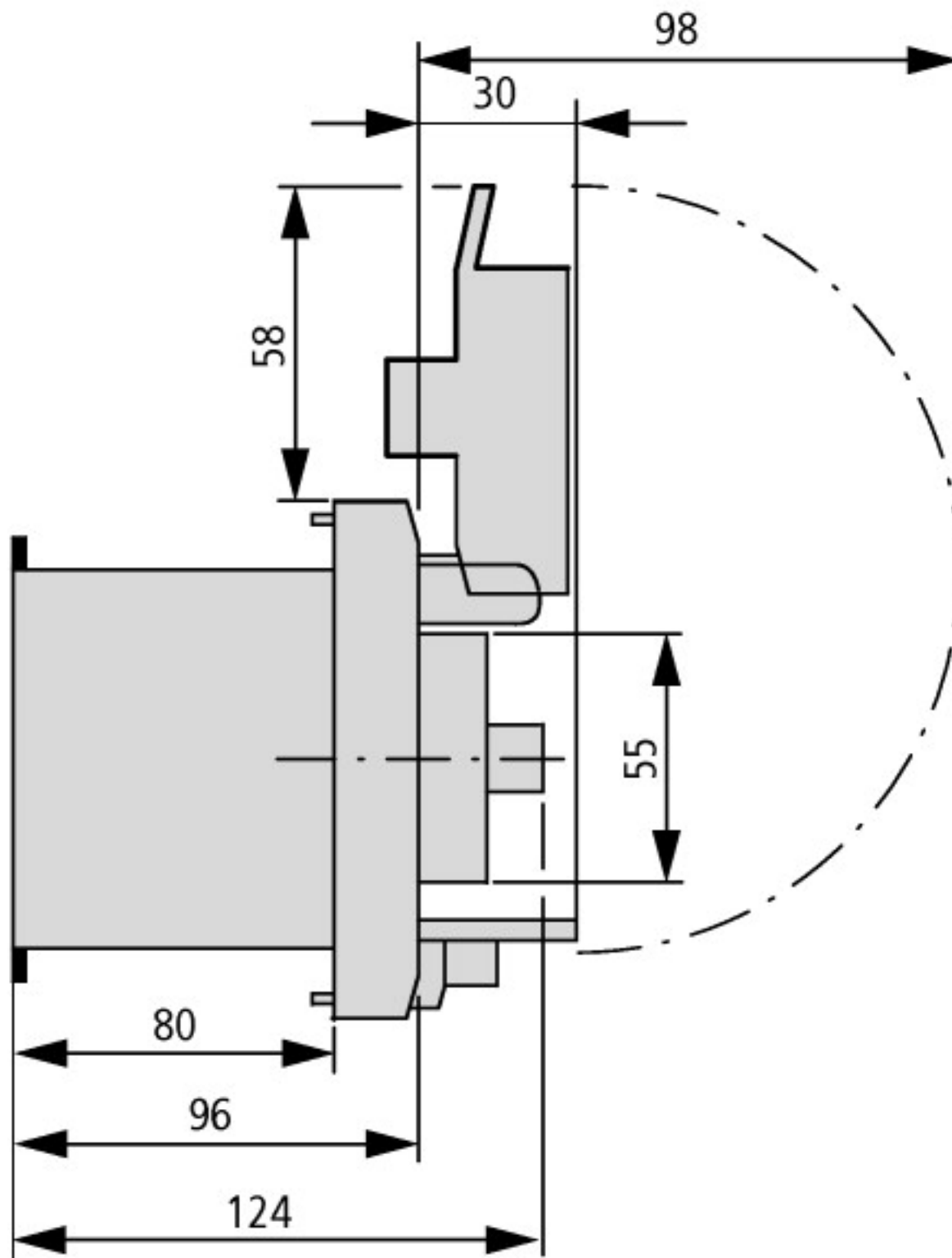
Insulated enclosure for flush mounting
