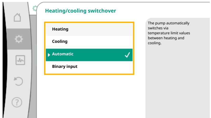
Fig. 56: Heating/cooling switchover_Automatic
