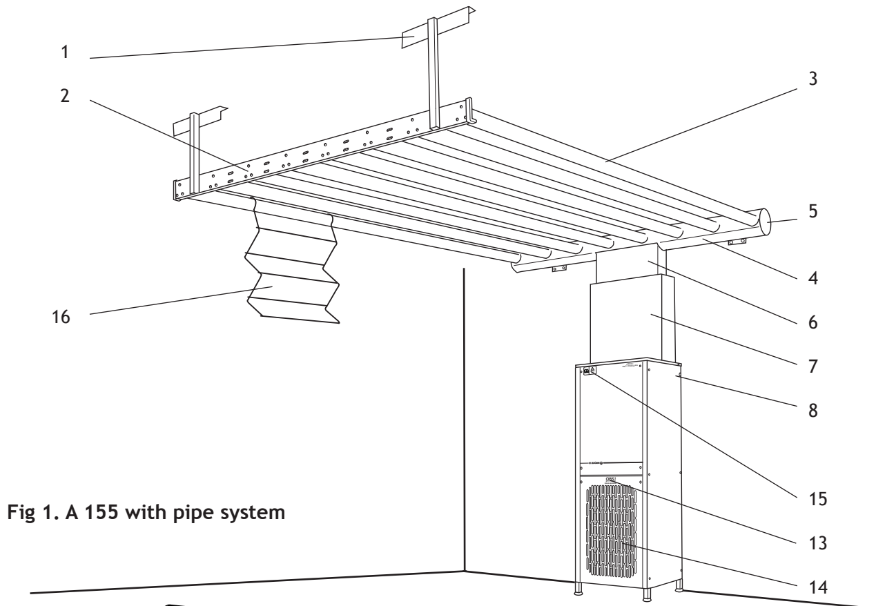
Fig 1. A 155 with pipe system
