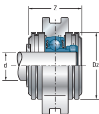
open SCOE closed SCCE with protective cap
