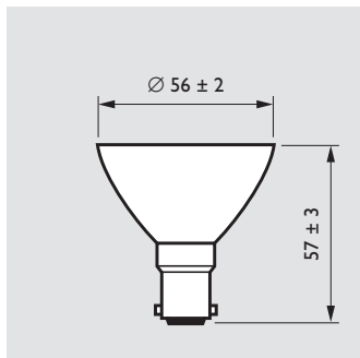
56 mm B15d/24x17 Dimensions in mm
