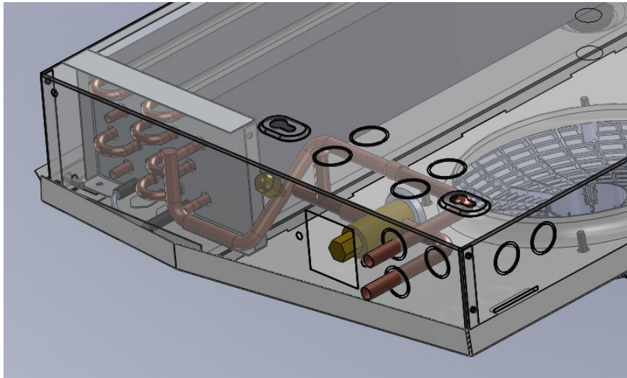
CS200 example of connection
