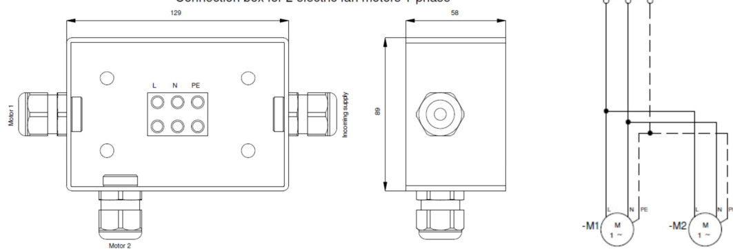
Connection box for 2 electric fan motors 1-phase
