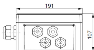
Connection box for electric defrost supply CD400
