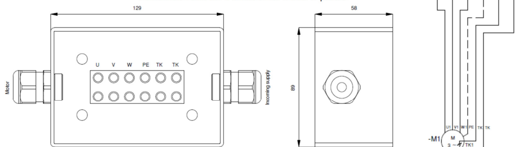
Connection box for 1 electric fan motor 3-phase
