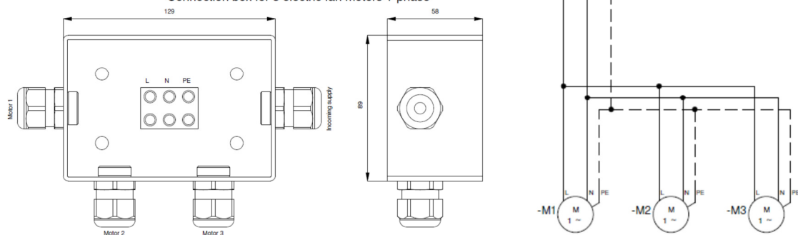
Connection box for 3 electric fan motors 1-phase
