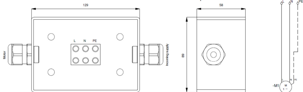
Connection box for 1 electric fan motor 1-phase
