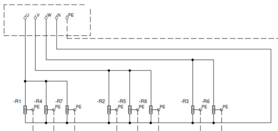
Connection box for electric defrost supply CD400
