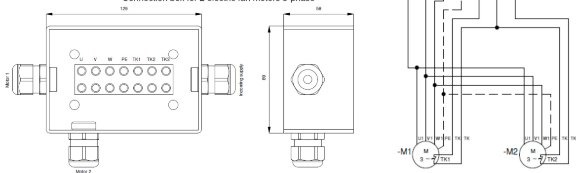
Connection box for 2 electric fan motors 3-phase
