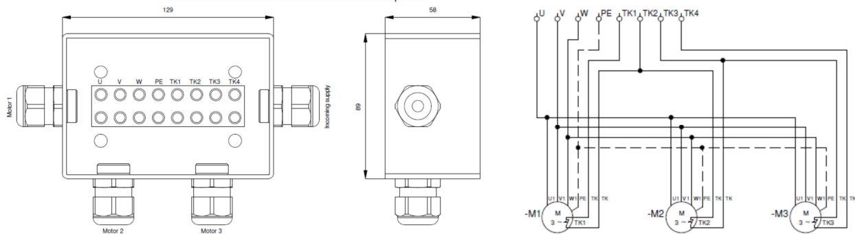
Connection box for 3 electric fan motors 3-phase
