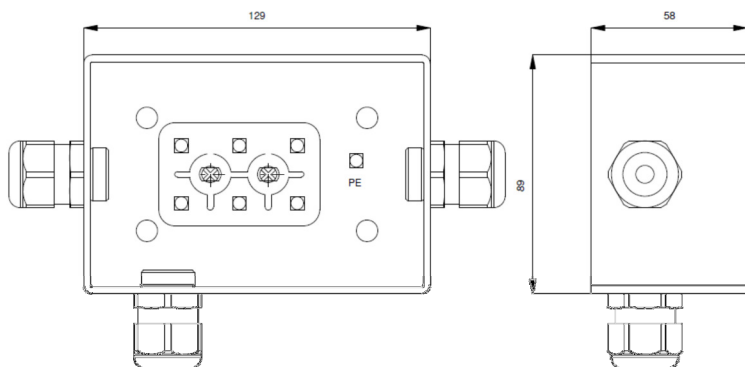
Connection box for electric defrost supply CD300
