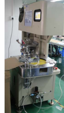
Auto-packing machine
