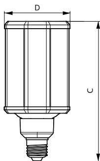
TForce LED HPL ND 4.5km E27 727 FR IP65
