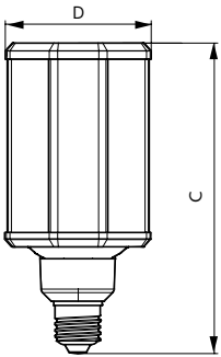
TForce LED HPL ND 5klm E27 740 CL IP65
