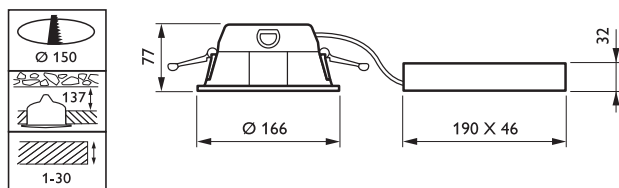
DN461B LED11S/830 PSE-E CU3 WH
