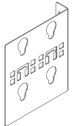
MOUNTING BRACKET, RIGHT
