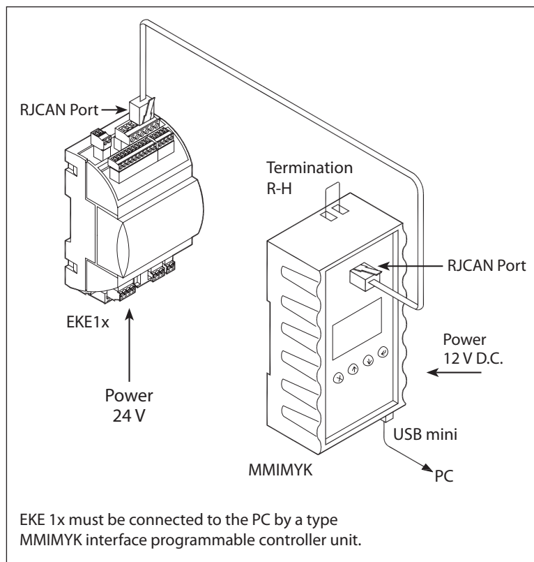
Fig 3. Connection for EKE using interface type MMIMYK (Code No. 080G0073)
