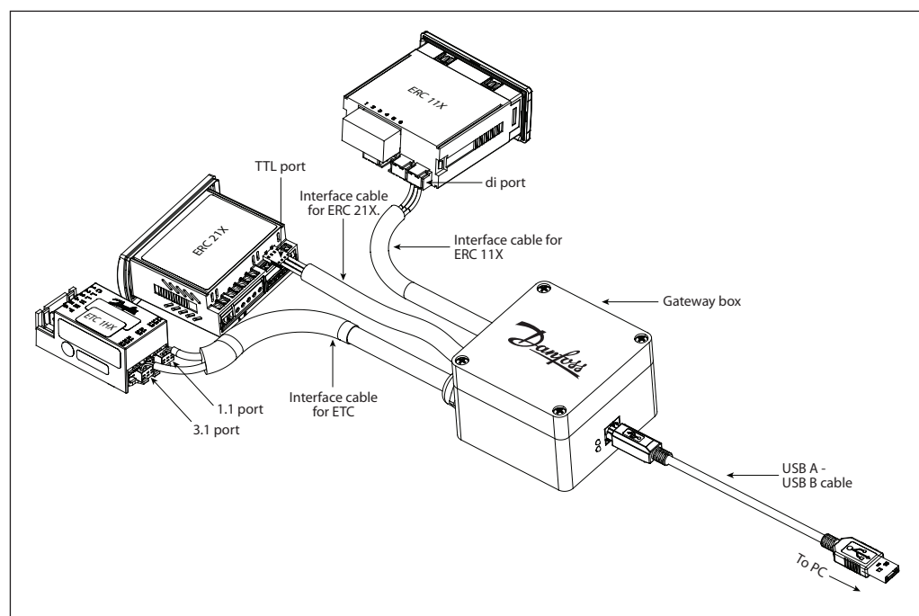
Fig 1. Connection for ERC and ETC using gateway box (Code No. 080G9711)
