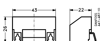
RC Element for contactors CI 6, 9, 12, 15, 16, 20, 25, 30
