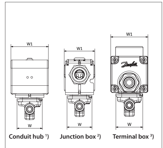
End view
