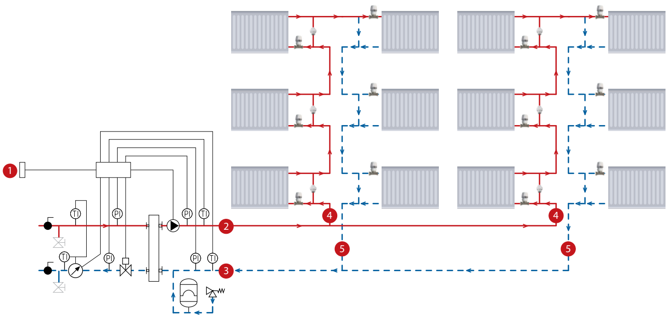
Fig 2: Measuring points
