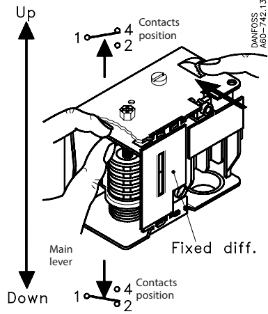
KP w/ manual reset
