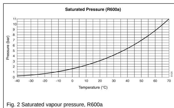
Fig. 2 Saturated vapour pressure, R600a
