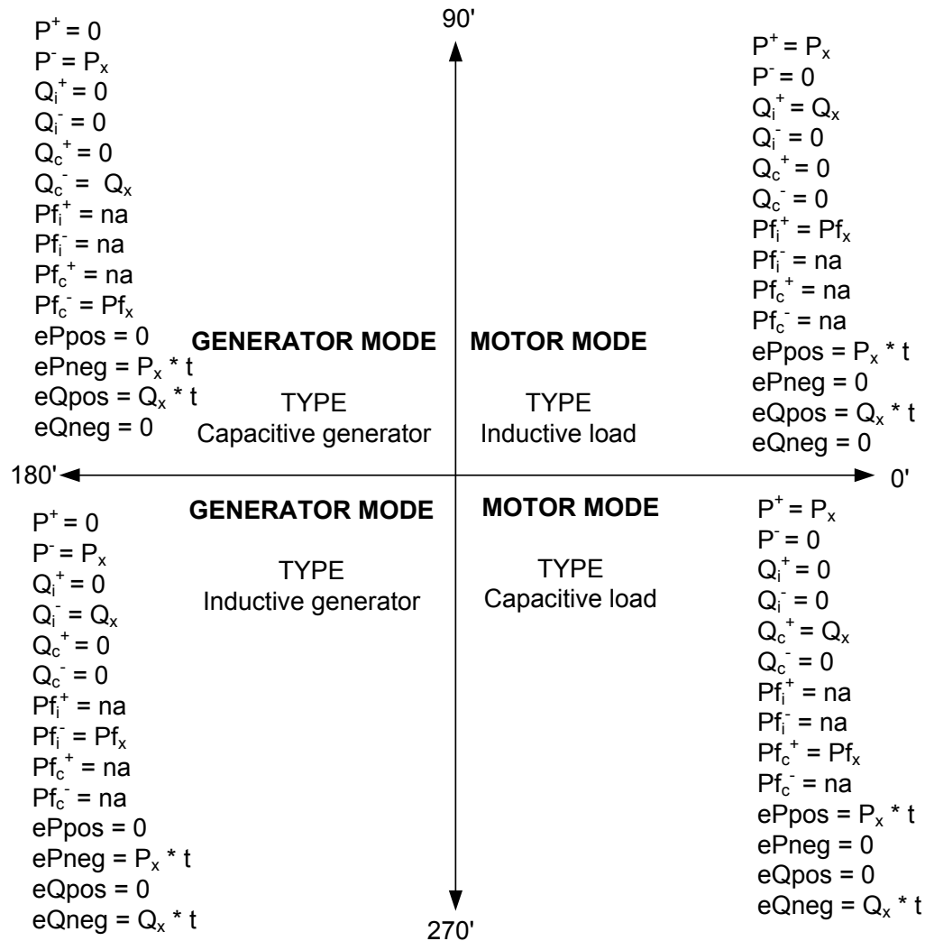
Figure 5.10: Motor/generator and inductive/capacitive phase/polarity diagram
