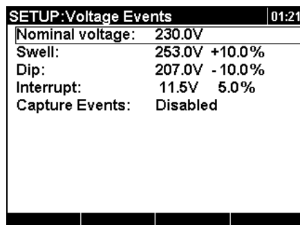
Figure 3.55: Voltage events setup screen.
