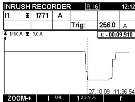
Figure 3.40: Captured inrush
