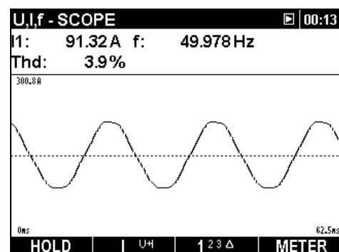
Figure 3.10: Current waveform
