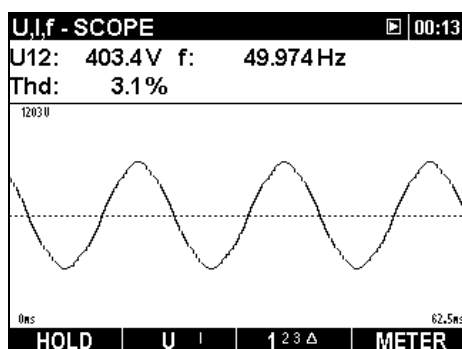
Figure 3.9: Voltage waveform
