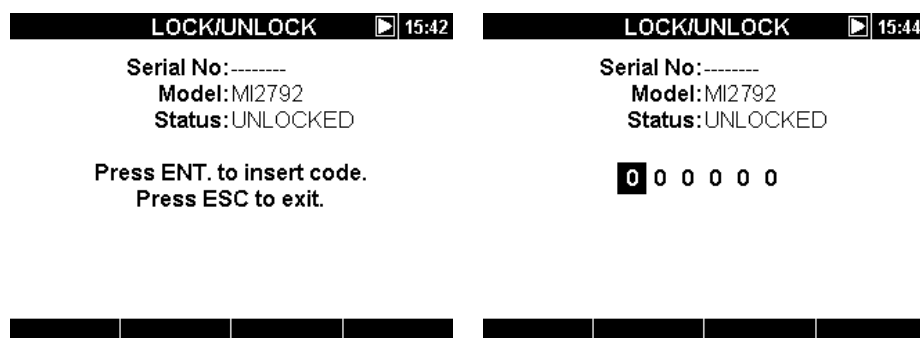
Figure 3.64: Lock/Unlock screen
