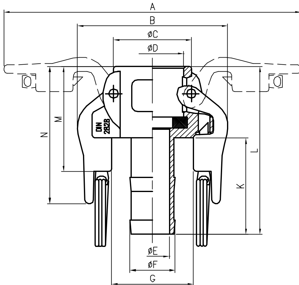
Dimensional sketch for Autolok, 733-CL
