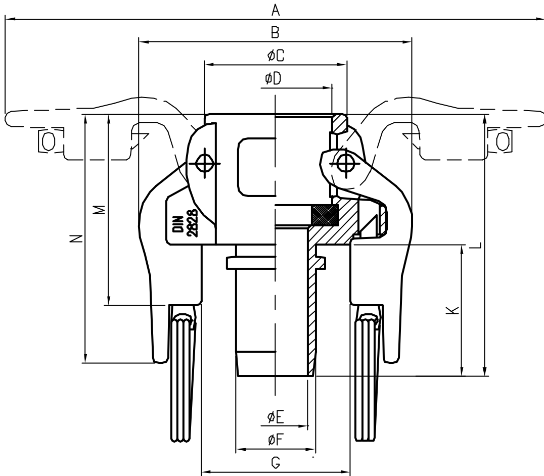
Dimensional sketch for Autolok, 733-CCL
