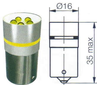
Socket BA 15s
