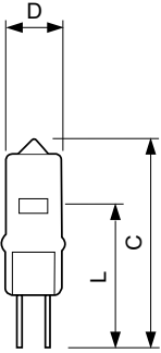
EcoHalo Capsule G4 12v14w CL B3000
