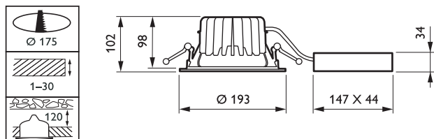
DN450B DLM1100/840 PSU-E WH
