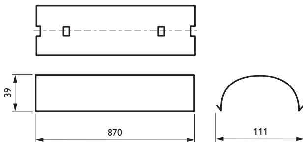
GMS122 21/39 R
