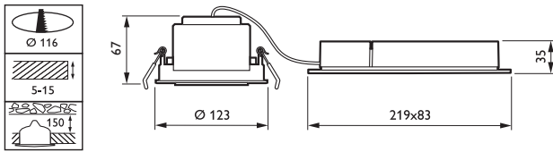
RS396B LED20-40-/830 PSU-E WH
