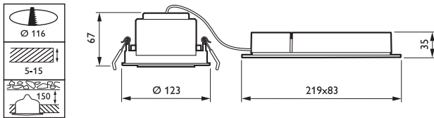
RS396B LED20-25-/830 PSU-E ALU
