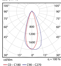
LED 5W 40°
