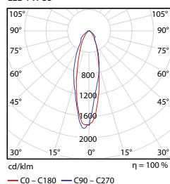
LED 7W 35°
