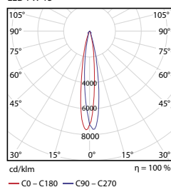
LED 7W 15°
