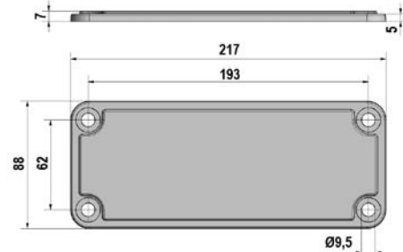
D-laippa
