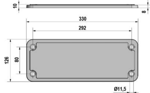
D-laippa
