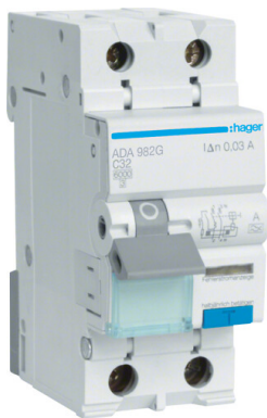
ADA982G
