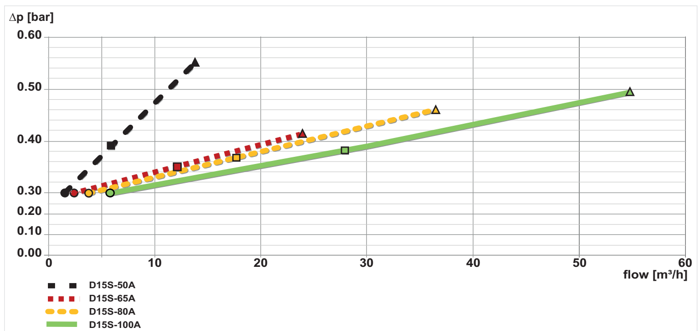
Fig. 2 Pressure drop within the valve in dependency of the flow rate and the used connection size (Sizes 50-100)
