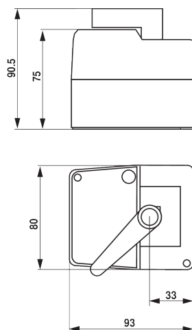
Dimensional drawings
