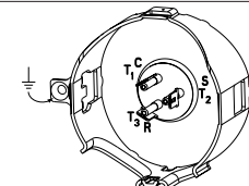
Quick connect spade terminals T and P terminal box type
