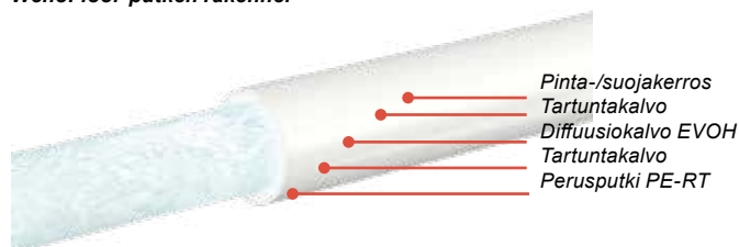
WehoFloor-putken rakenne:
