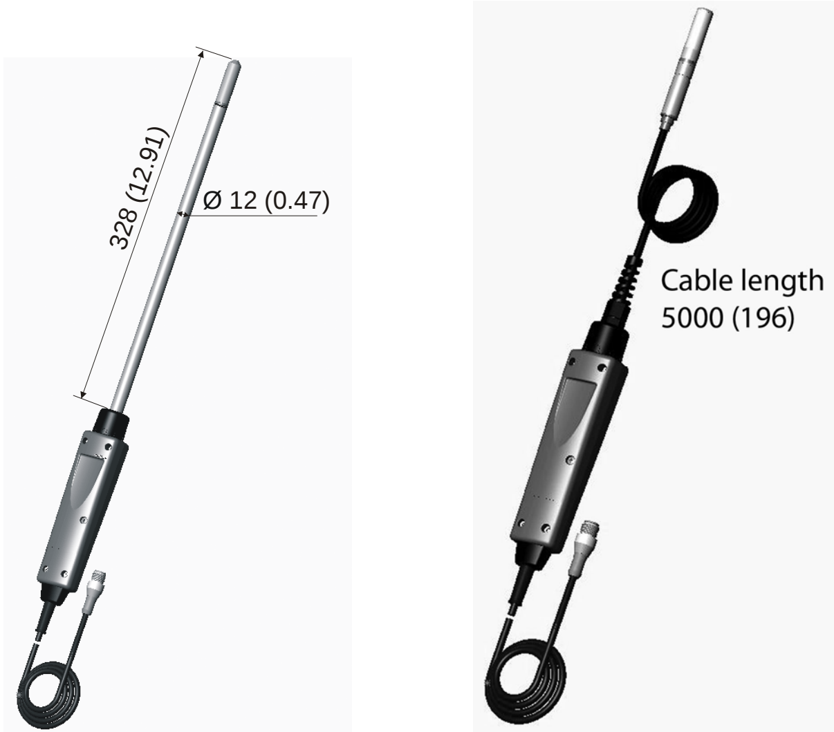
HMP76 Probe
