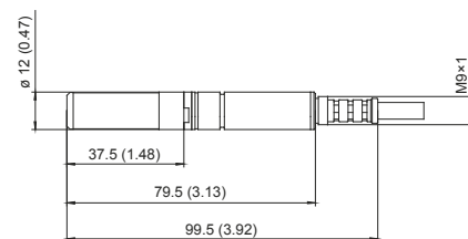
HMP77 probe
