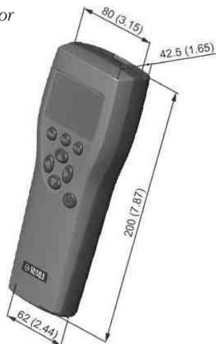
HMP75 probe
