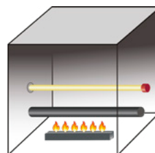
27 m³ cube smoke chamber
