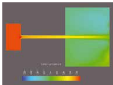
Conventional sound baffle The CFD simulation image on the left shows the pressure loss profile of the conventional sound baffle available on the market today
