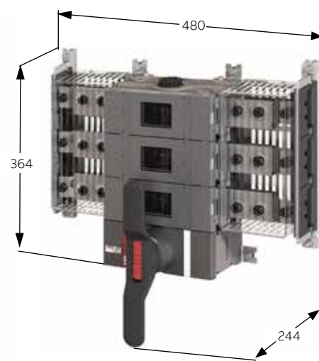
LBOD 1600
