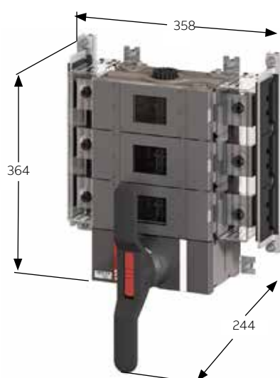
LBOD 1000
