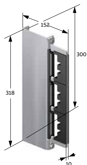
MSB 316/100
