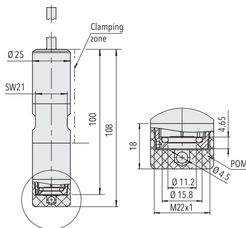
Standard version
