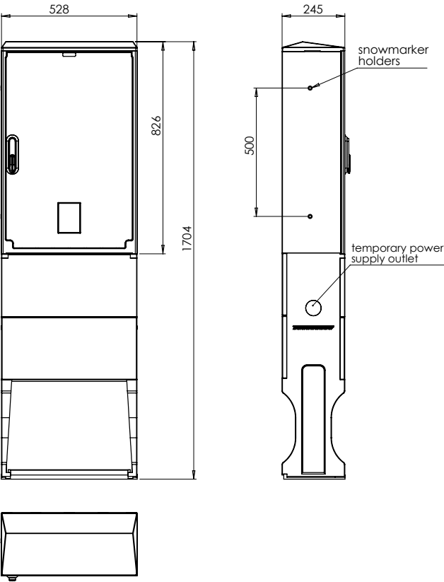
OKKJK-P 400A 53X80 BC+3x160
