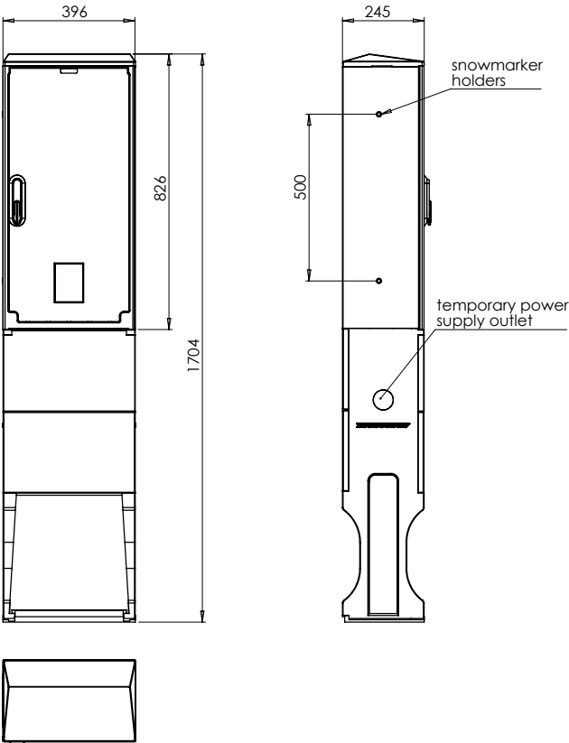
OKKJK-P 250A 40X80 BC+2X160
