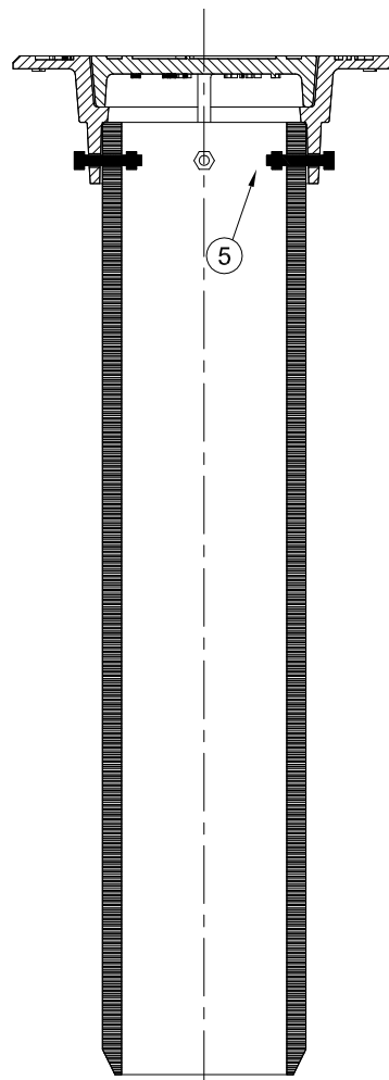
SECTIONAL VIEW Y-Y
